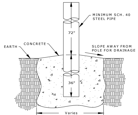
POLE INSTALLATION DETAIL
